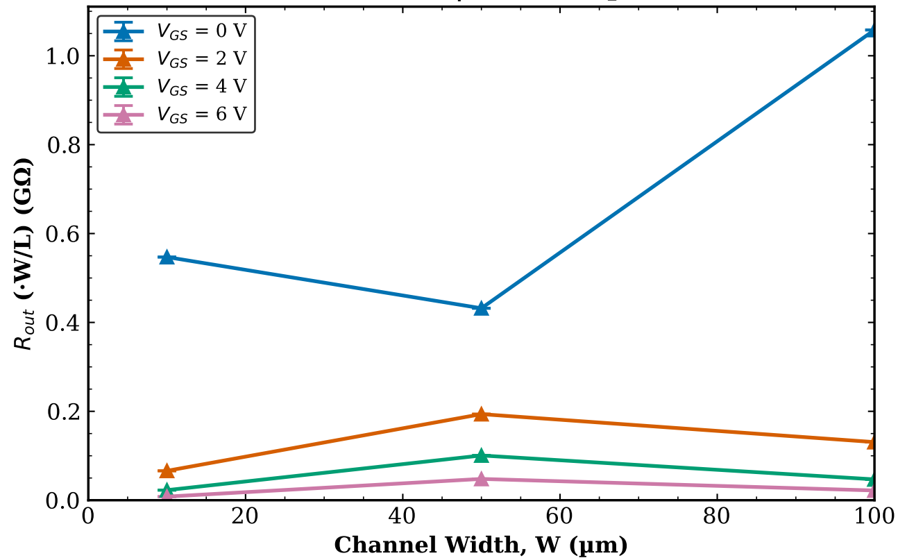
TFT1 Transistor 1 R_{out} vs W | L = 160\text{ }\mu\text{m}
